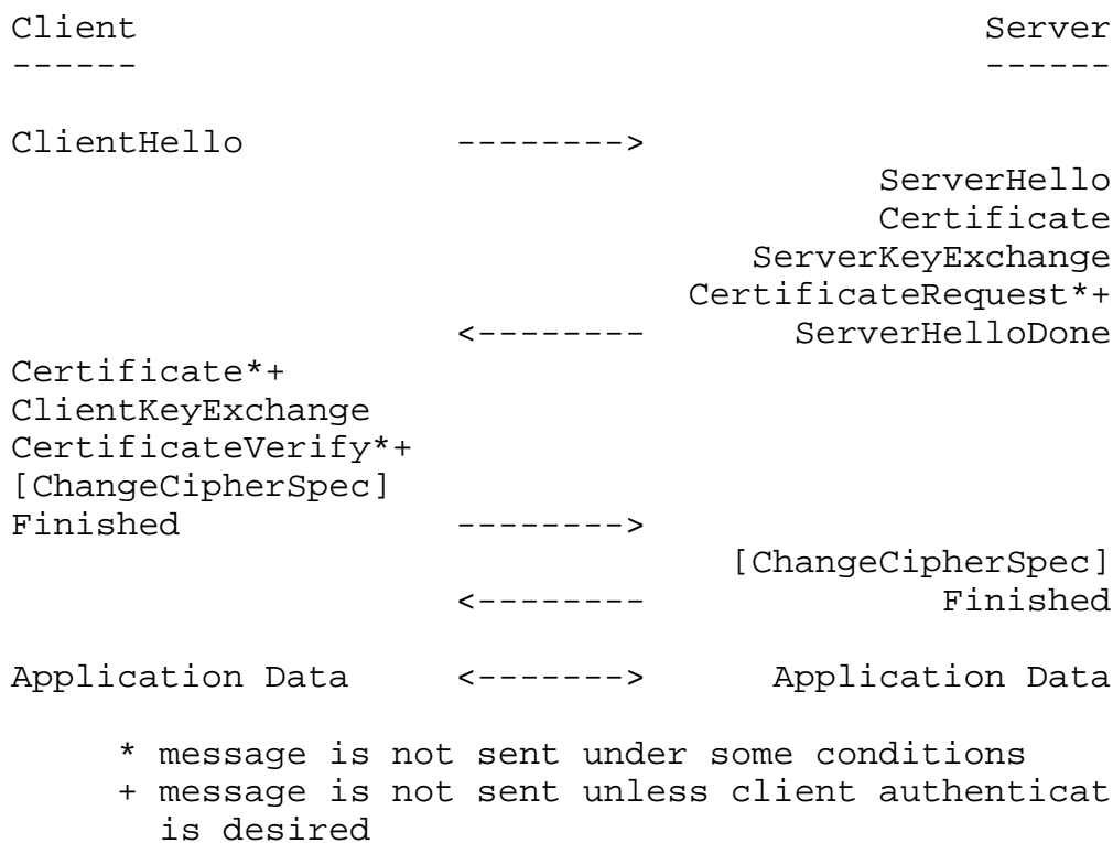
Figure 1: Message flow in a hybrid TLS handshake
