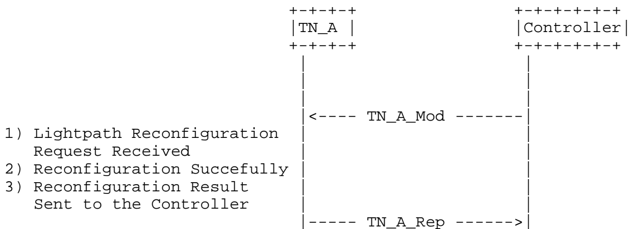
Figure 8: Lightpath Reconfiguration Reply (Success) from TN_A
