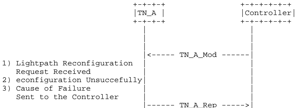
Figure 9: Lightpath Reconfiguration Reply (Failure) from TN_A
